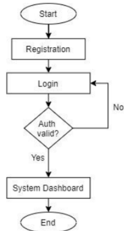
Fig. 3. Authentication flowchart
