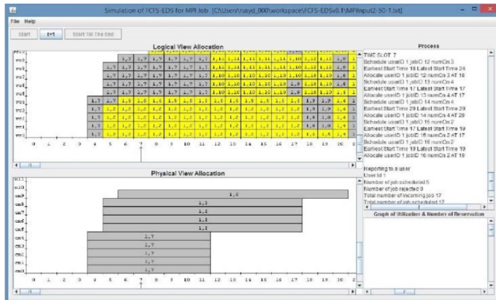
Simulation of FCFS-EDS scheduling for MP1job
