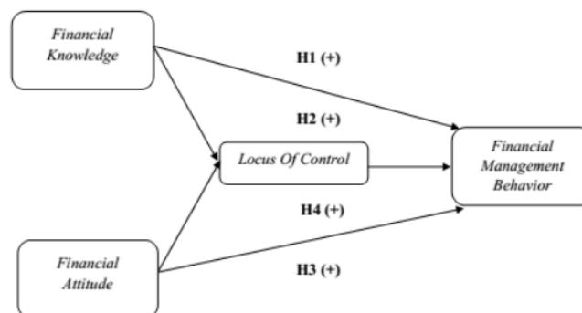
Gambar 1. MODEL PENELITIAN
