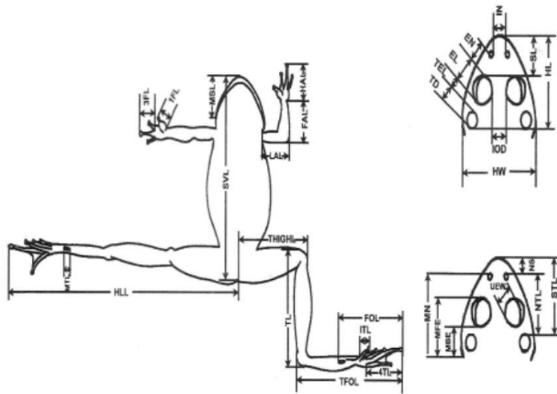
Fig. 1. Amphibian morphometric measurements (Tjong et al. , 2013)
