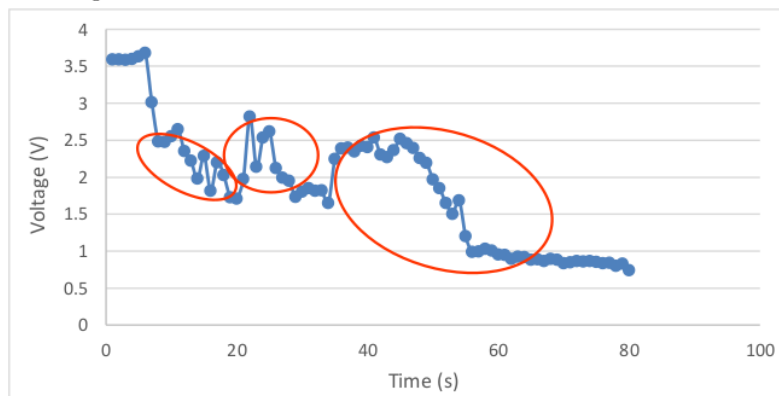
Figure 6. The result of output voltage fiber optic
