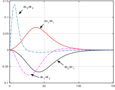
(a) Sensitivity functions X_r := \frac{\partial X}{\partial r} .
