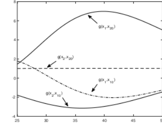
(b) Generalized sensitivity functions g(X, x_0) .
