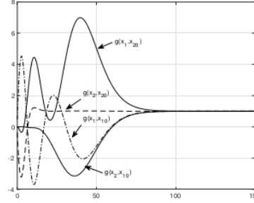
(b) Generalized sensitivity functions g(X, x_0) .
