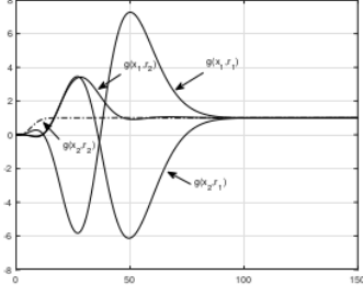
(a) Generalized sensitivity functions g(X, r) .
