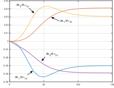
(b) Sensitivity functions X_\alpha := \frac{\partial X}{\partial \alpha} .
