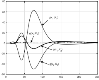
(b) Generalized sensitivity functions g(X, K) .
