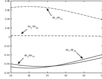
(a) Traditional sensitivity functions X_{x_0} := \frac{\partial X}{\partial x_{x_0}} .
