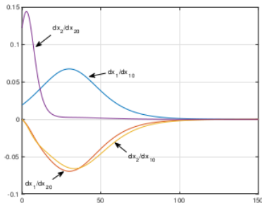
(b) Sensitivity functions X_{x_0} := \frac{\partial X}{\partial x_0} .
