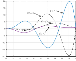
(b) Generalized sensitivity functions g(X, r) .
