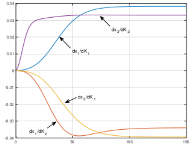
(a) Sensitivity functions X_K := \frac{\partial X}{\partial K} .
