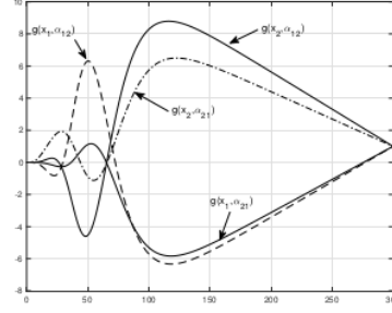
(a) Generalized sensitivity functions g(X, \alpha) .
