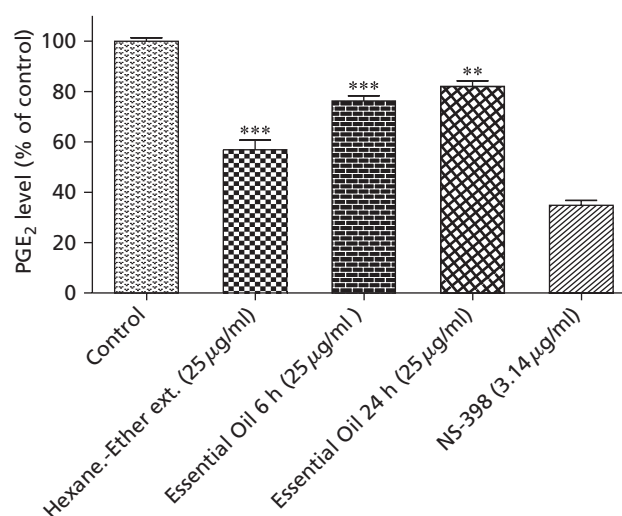
Figure 1 Inhibitory effect of the B. marginatum essential oils and hexane–ether extract on PGE 2 production in MiaPaCa-2 cells. Effect was studied using ELISA immunoassay. Data are presented as means \pm SEM from three independent experiments. ** P < 0.01 , *** P < 0.001 compared with the control.
