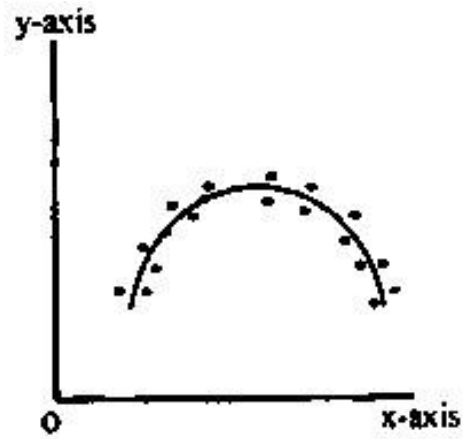
Model Non-Linier
