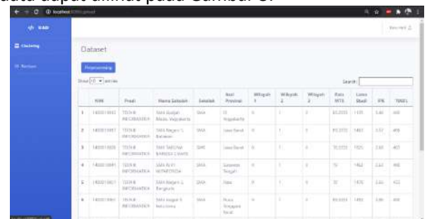
Gambar 3. Load Dataset
