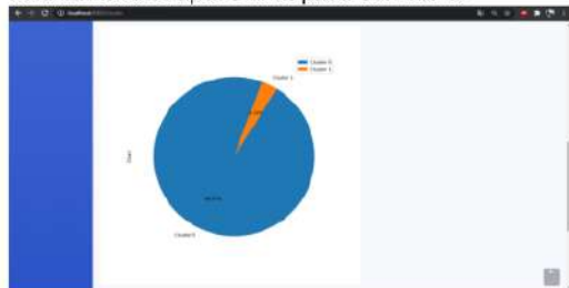
Gambar 6. Chart
