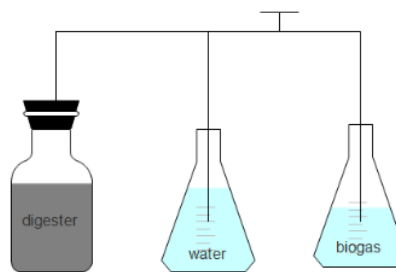
Figure 1. Schematic Showing Water Displacement Method
