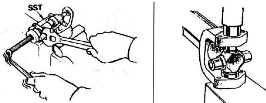
Gb. 9. Memasang spider bearing
