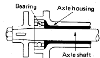
Gb. 5. Poros tipe semi floating
