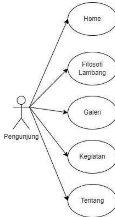
gambar 3.1 use case diagram
