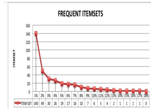
Fig. 3. Correlation of minimal support and number of frequent itemset
