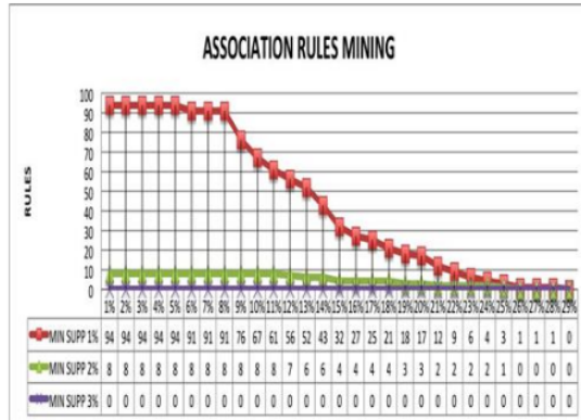
Fig. 4. Experiment result of determination min_sup and min_conf
