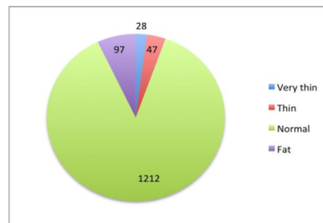
Fig. 3. Data distribution of nutritional status in body height per age
