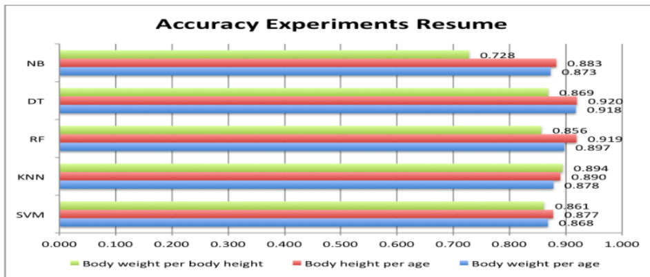
Fig. 5. Average of experiments accuracy
