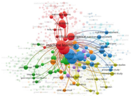
Fig. 11. Co-word analysis for malnutrition words
