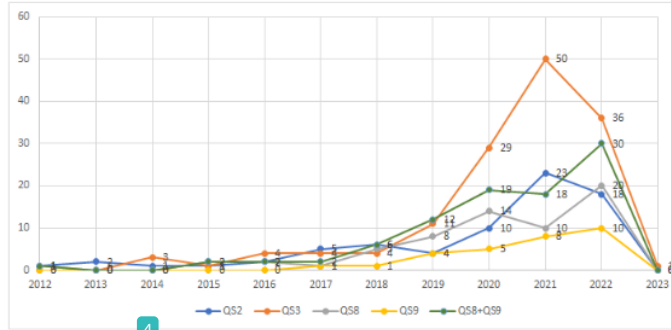
4 Fig. 2. Number of publications per query string
