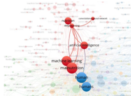
Fig. 12. Co-word analysis for artificial intelligence words
