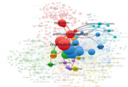
Fig. 10. Co-word analysis for artificial intelligence words
