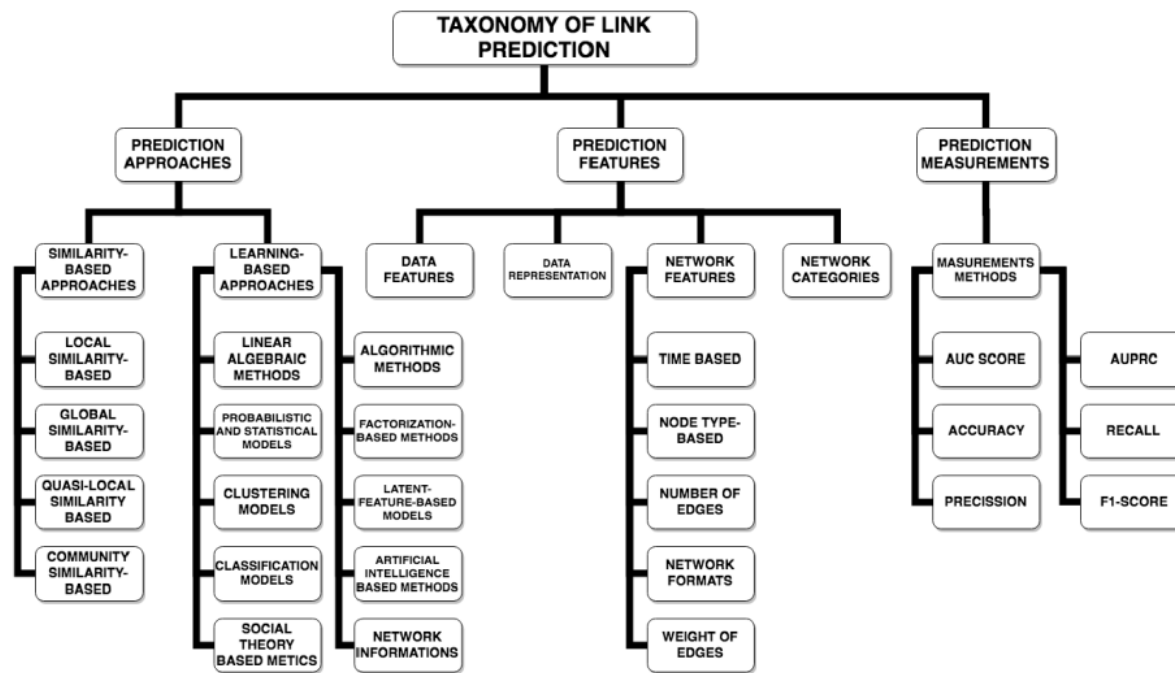
FIGURE 1. Taxonomy of link prediction.
