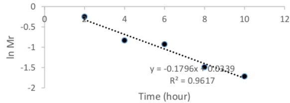
Figure 2. Effective Moisture Diffusivity
