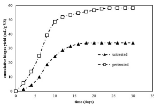
Figure 2. Cumulative biogas yield during 30 days
