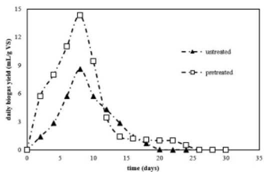
Figure 1. Daily biogas yield during 30 days
