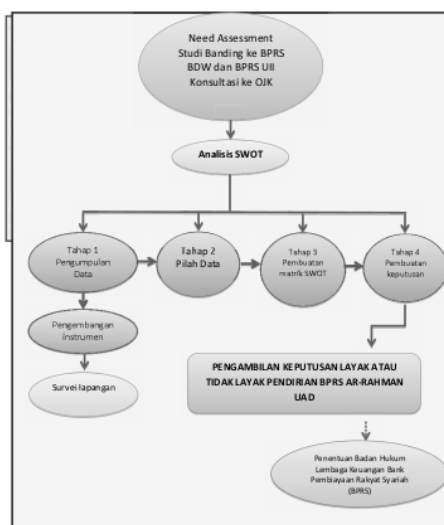
Gambar 1 Rerangka Penelitian
