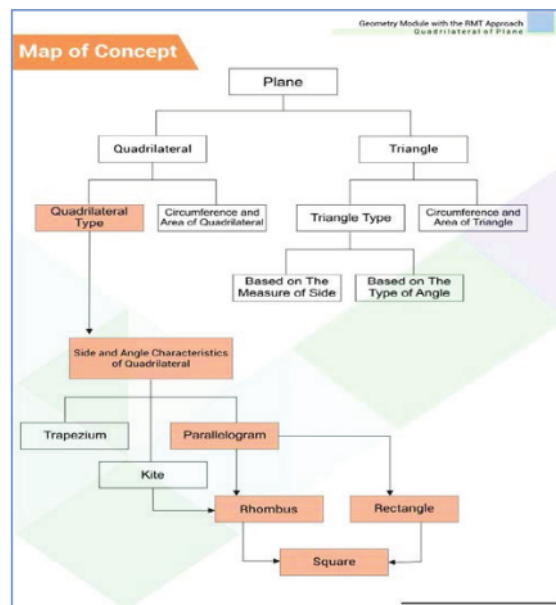
FIGURE 2. The map of concept quadrilateral
