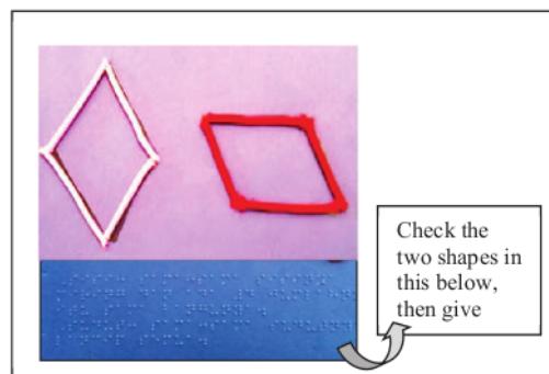
FIGURE 4. The problems of quadrilateral relations
