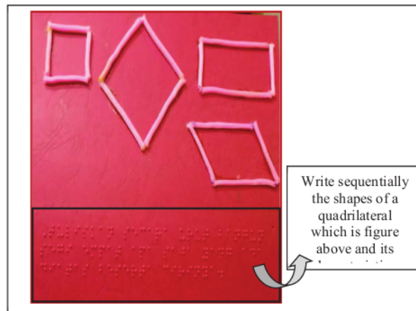
FIGURE 3. The problem of labeling and visualizing quadrilateral
