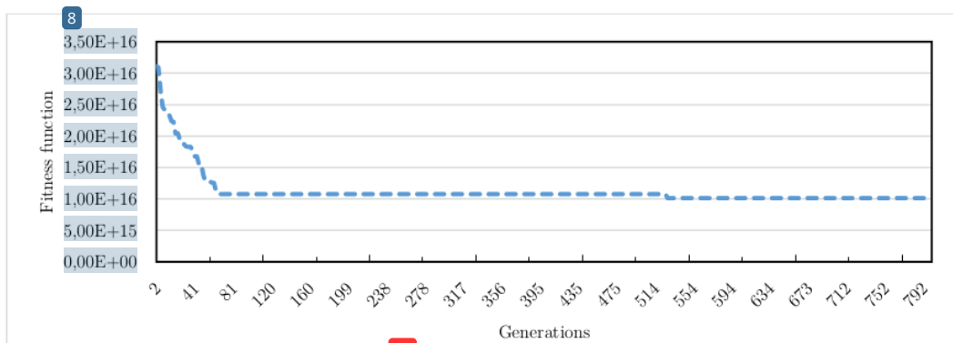
Fig. 8 The search process of GA (test-4) in finding the optimal solution for the DLS model with a constrained inventory capacity.
