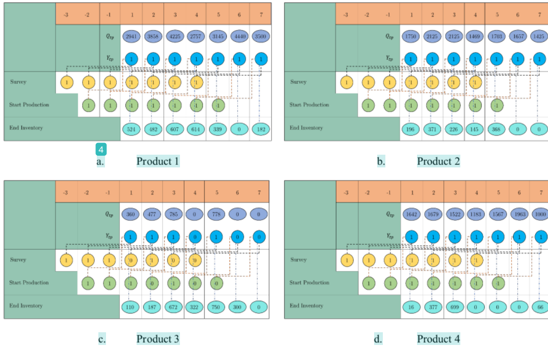
Fig. 10 The impact of the production decision under four products for the DLS model with unconstrained inventory capacity extend to the management of process business in bread making, encompassing both production volume and binary production decisions
