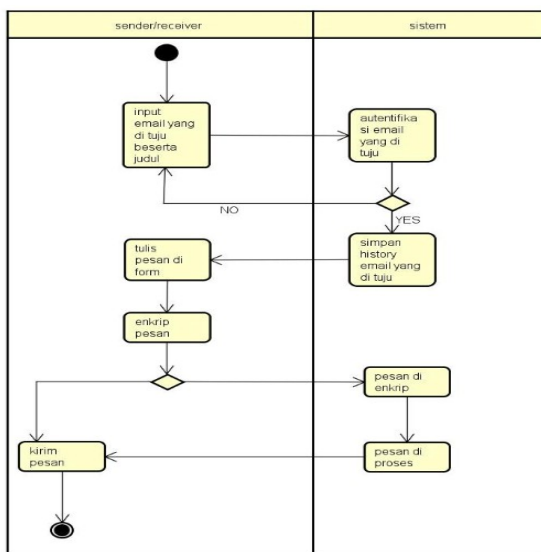
Gambar 3. Activity diagram menulis pesan
