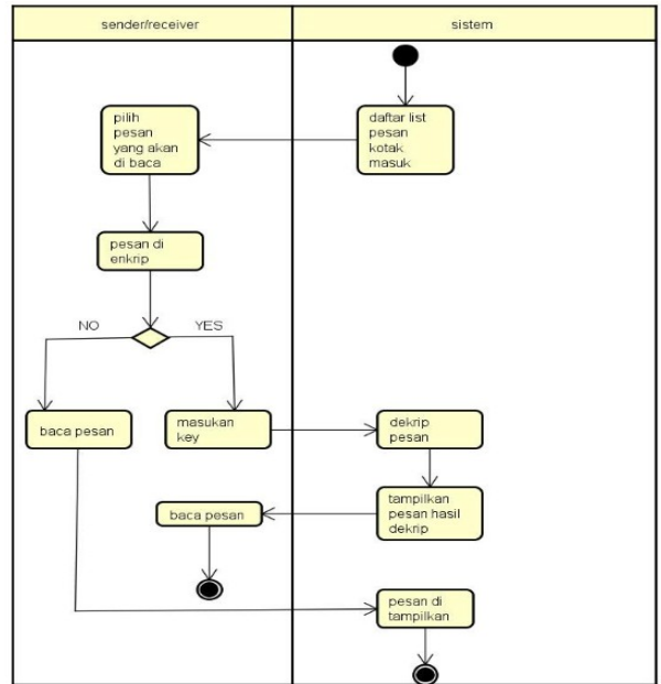
Gambar 4. Activity diagram proses baca email
