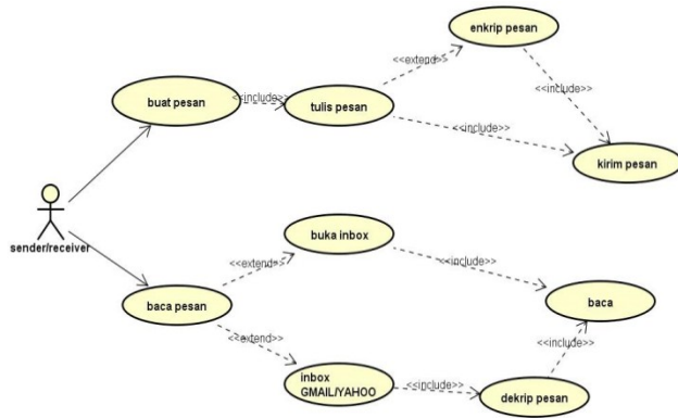
Gambar 2. Use Case diagram K-Email
