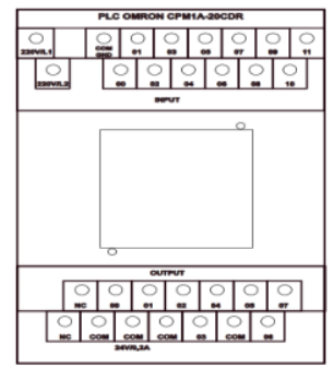
Figure 3. Trainer Design
