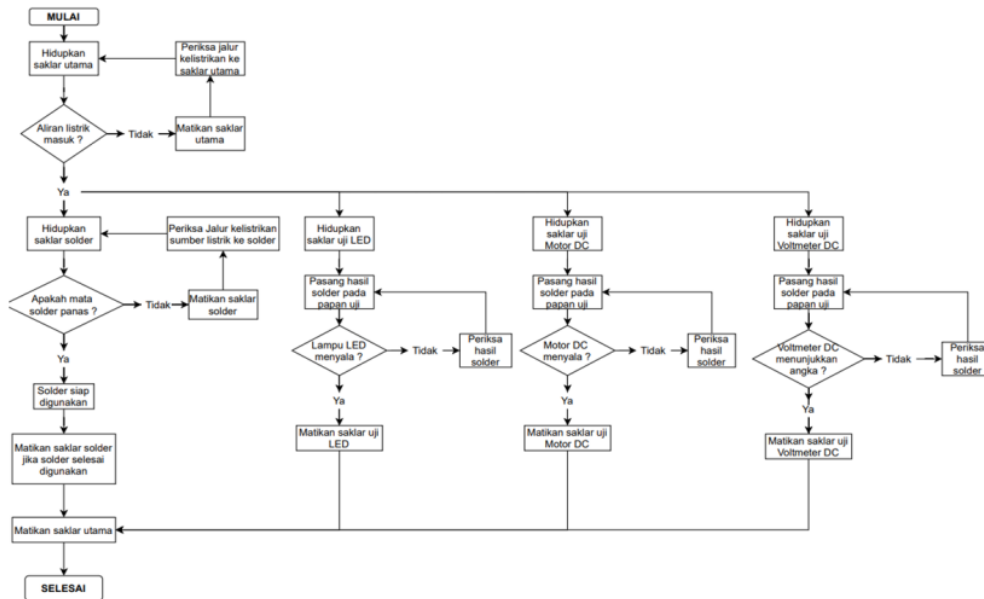
Gambar 10. Diagram Alir Trainer Kit PCB Solder
