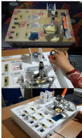
Gambar 5. Hardware trainer kit PCB Solder
