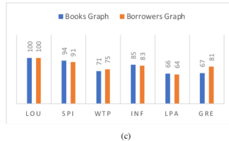
Figure 4. Distribution on bipartite graph: (a) Community size (sc) Distribution on books graph; (b) Community Size (sc) distribution on borrower graph; (c) Community fit.
