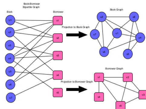
Figure 3. Projection of book-borrower graph.
