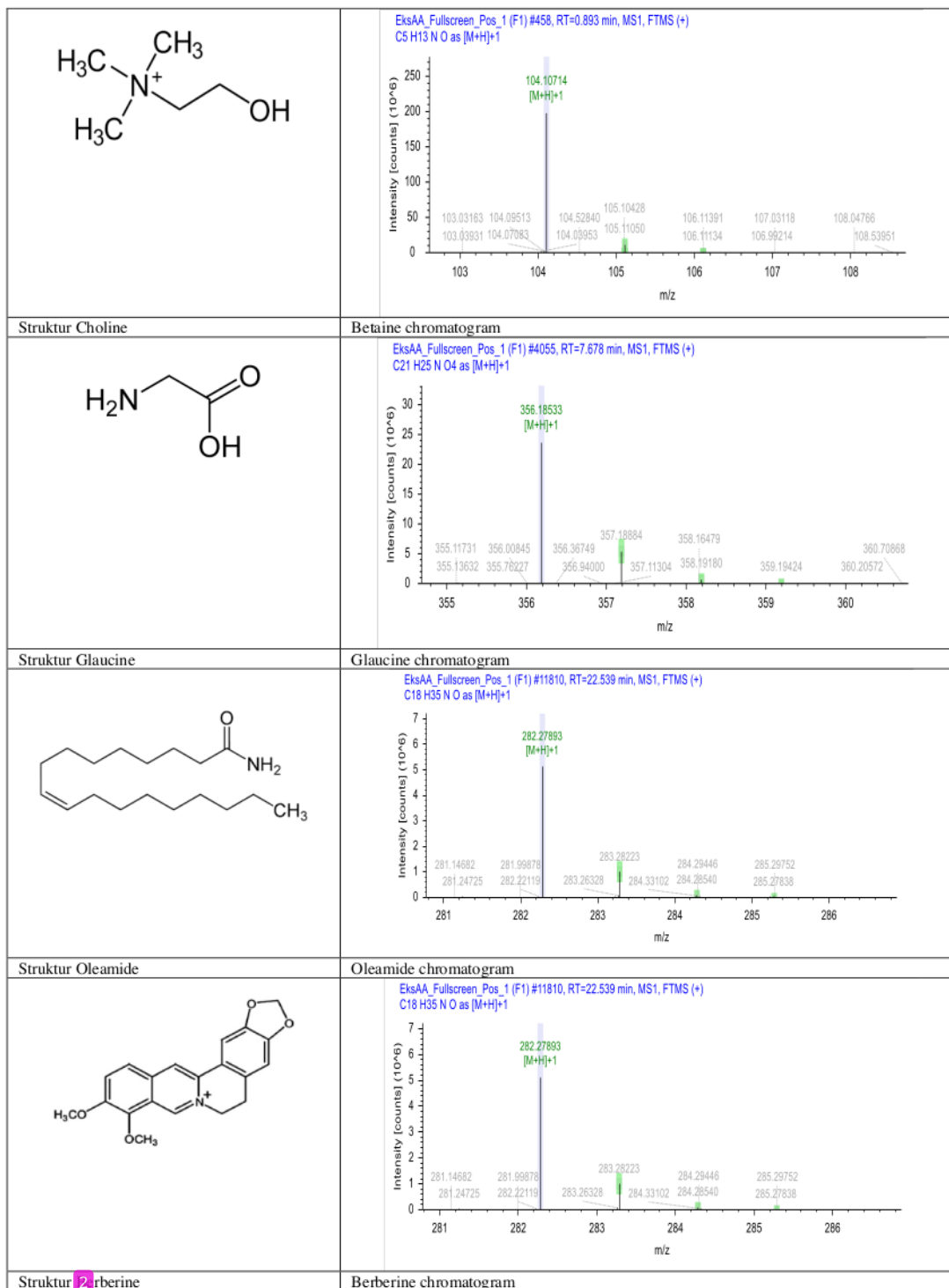
Figure 2: Analysis of the chemical content of the ethanol extract of Fibraurea tinctoria , by using LC-HRMS
