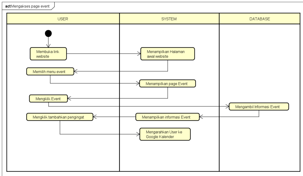
Gambar 4. 16 Activity user tokosaudarasbc mengakses page event
