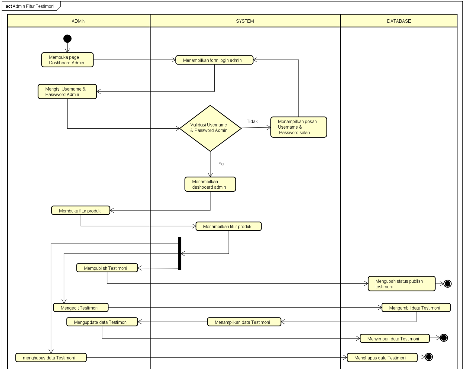
Gambar 4. 9 Activity Admin asaprimaniaga fitur testimoni
