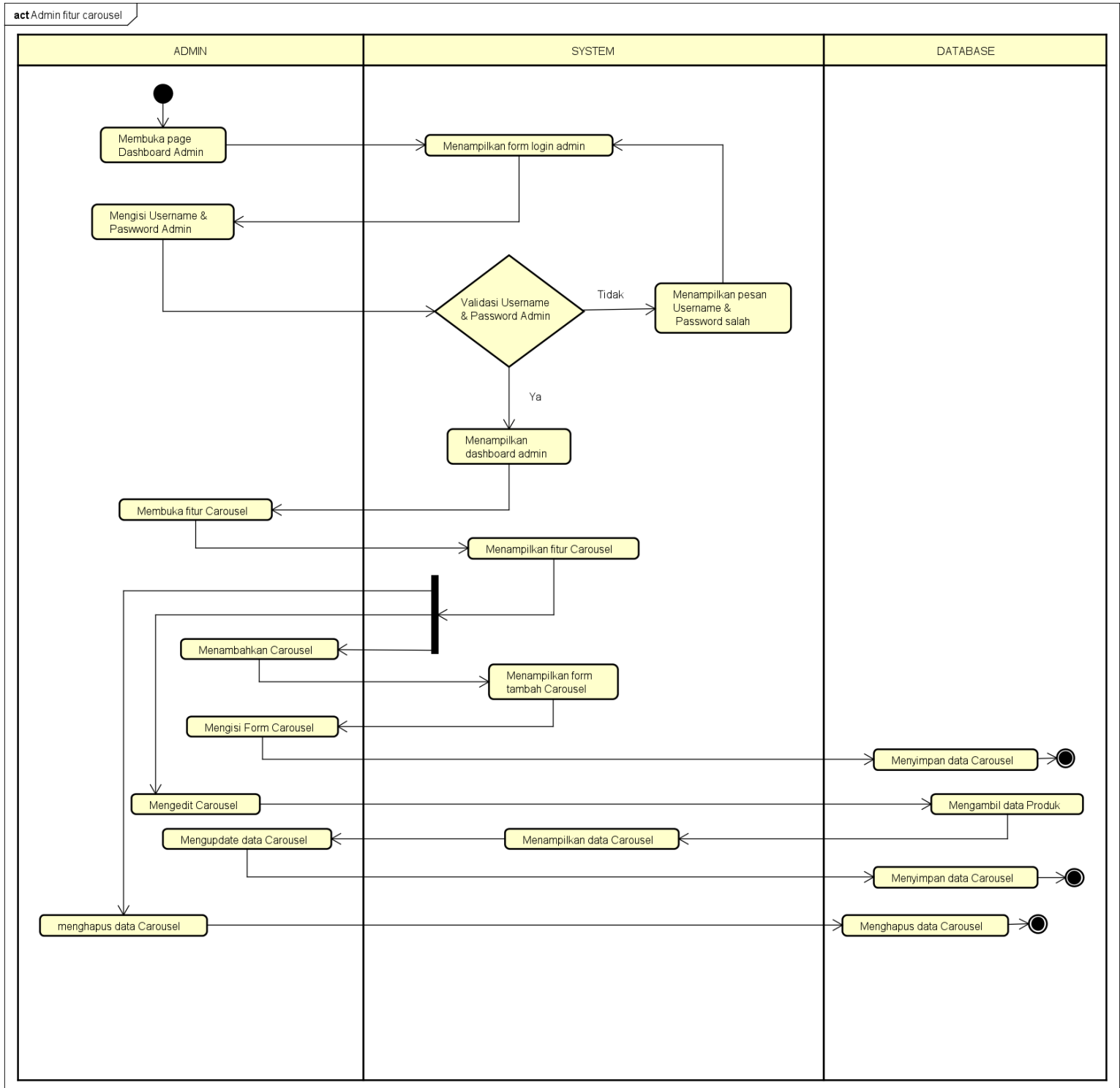
Gambar 4. 19 Activity diagram admin tokosaudarasbc fitur carousel
