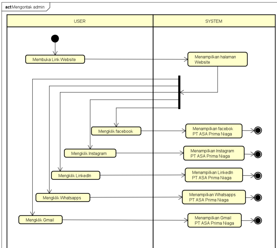
Gambar 4. 5 Activity User asaprimaniaga mengontak admin
