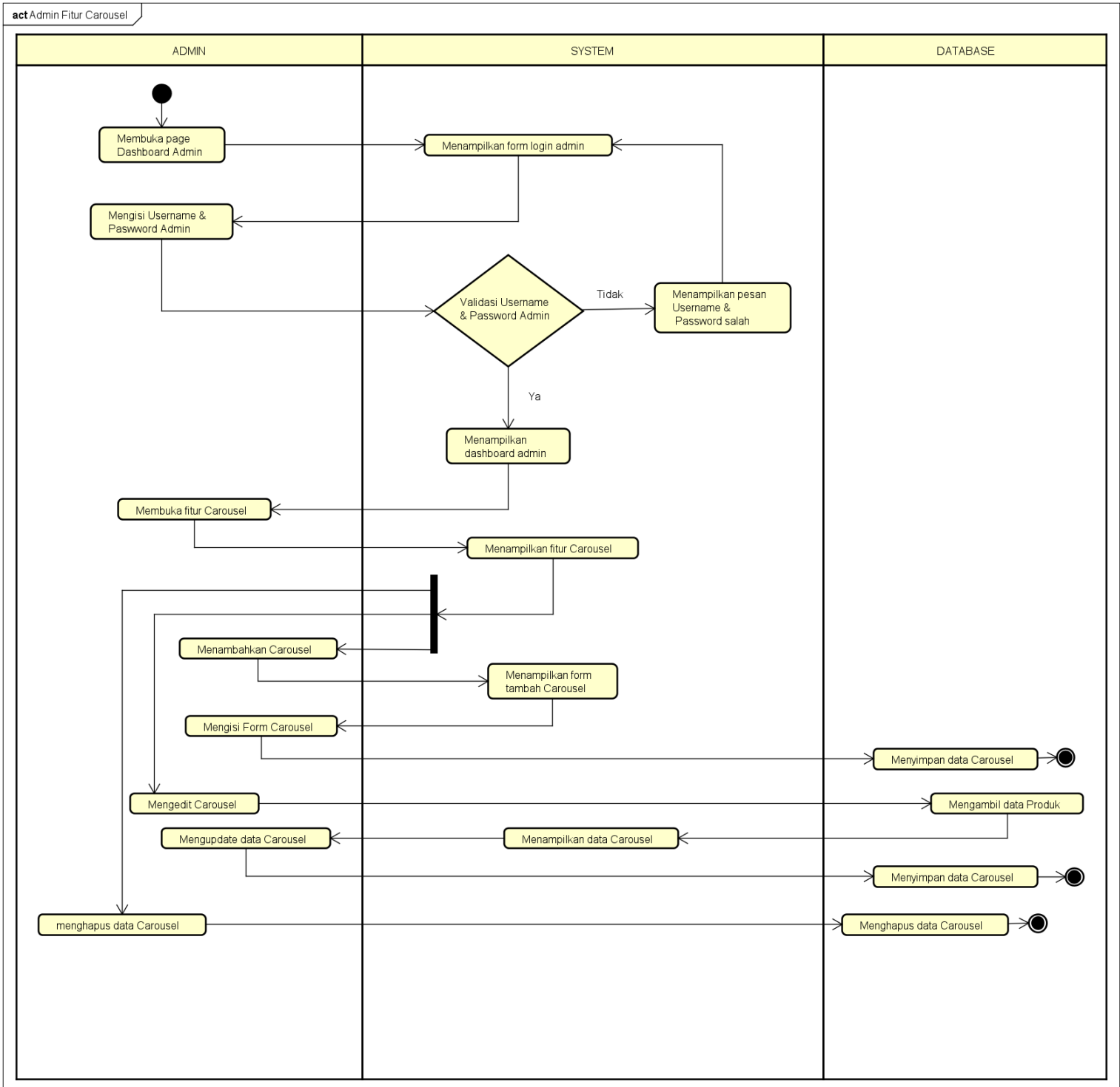
Gambar 4. 7 Activity Admin asaprimaniaga fitur carousel
