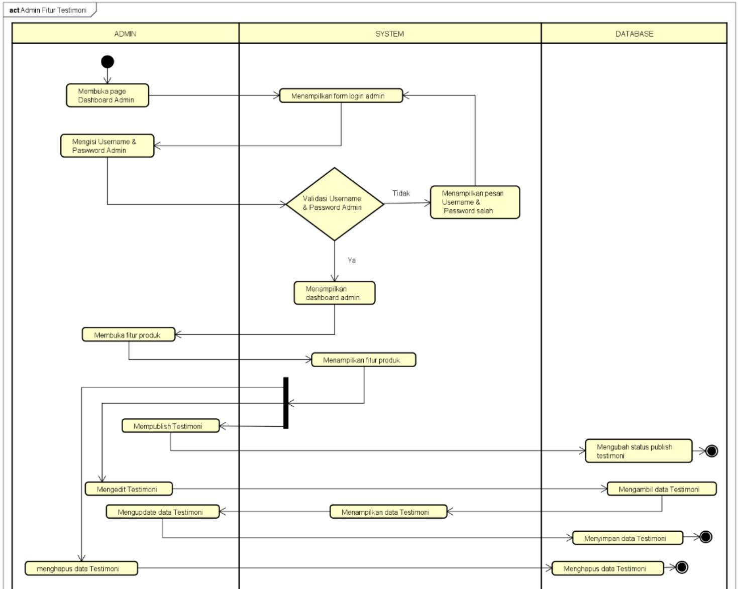
Gambar 4. 3 Activity User asaprimaniaga membuka page testimoni
