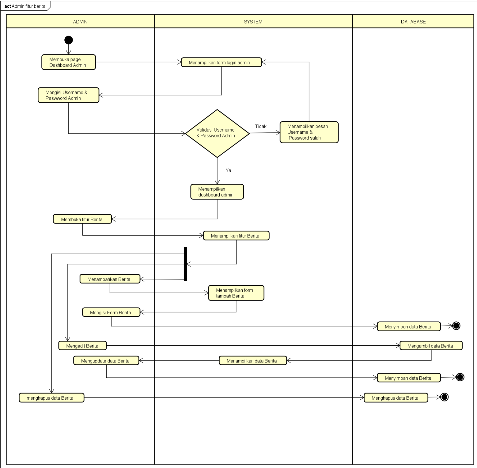
Gambar 4. 18 Activity diagram admin tokosaudara sbc fitur berita
