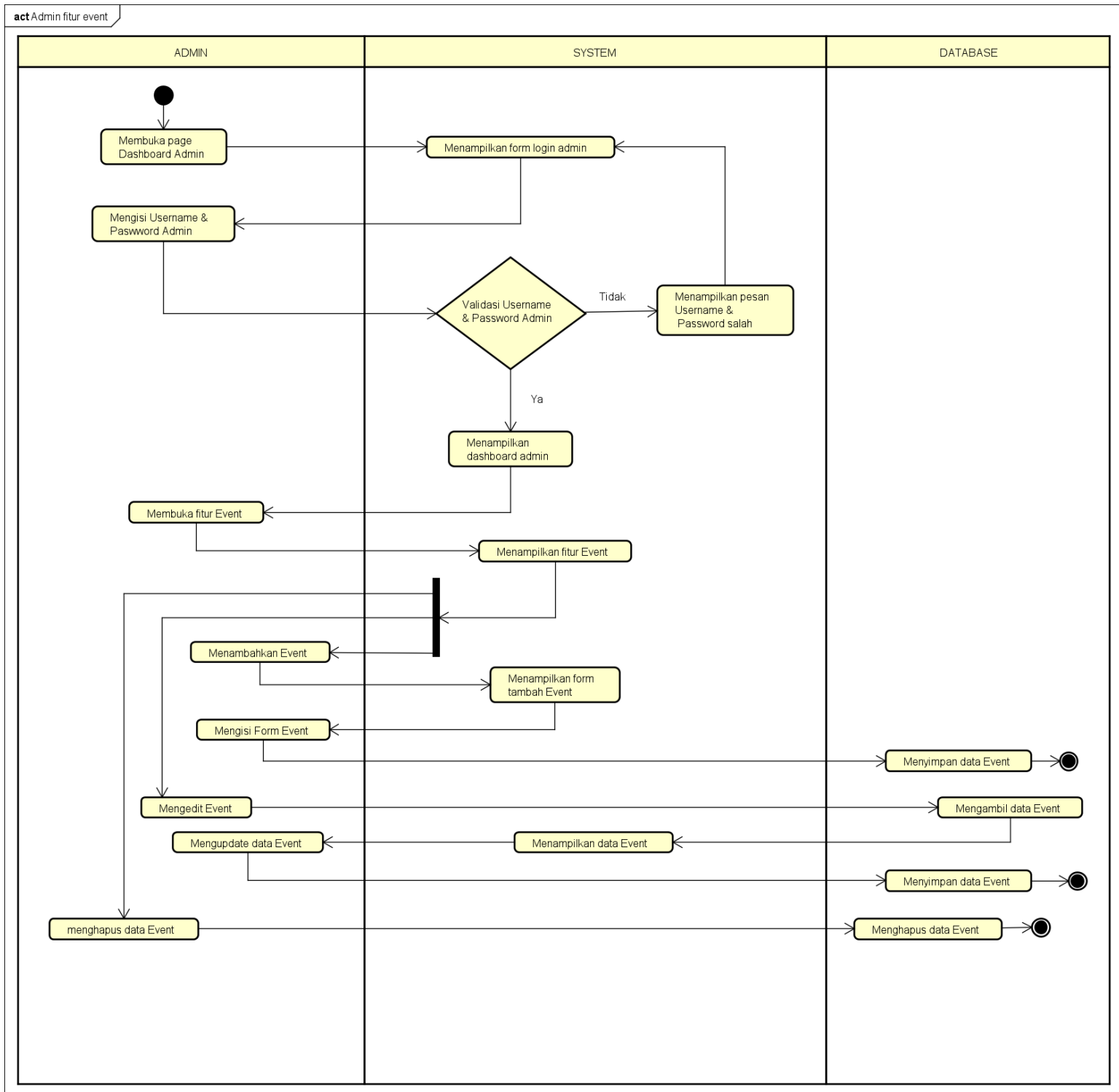
Gambar 4. 20 Activity diagram admin tokosaudarasbc fitur event
