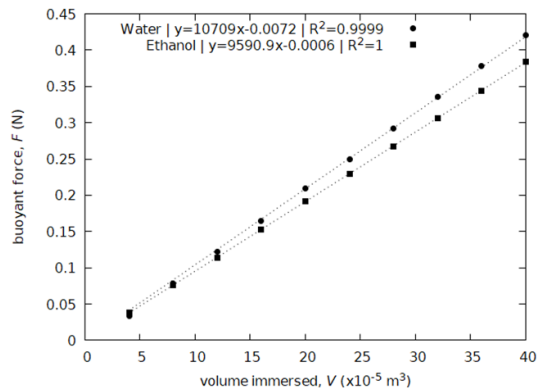
Figure 9. The graph of the relationship between the volume of objects immersed with buoyant force on objects.
