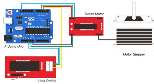
Figure 3. Schematic diagram of stepper motor control circuit.
