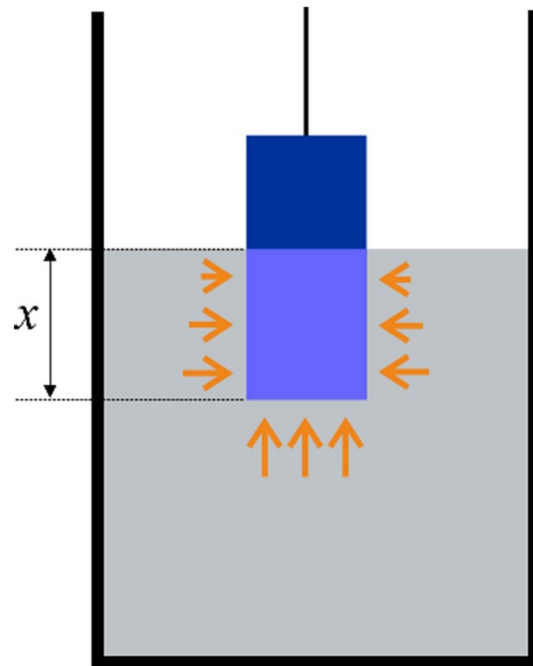
Figure 1. Forces due to pressure acting on the surface of a partially immersed body. Reprinted from [6], with the permission of AIP Publishing.
