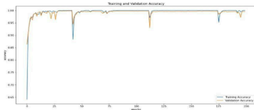
Fig 5. Accuracy Results
