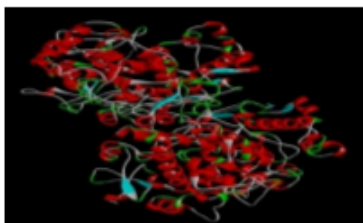
Gambar 2. Struktur 6COX cyclooxygenase-2 (prostaglandin synthase-2) complexed with a selective inhibitor, sc-558 in 1222 space group belum di preparasi
