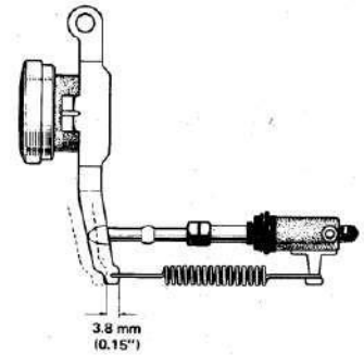
Gb. 17. Release silinder dan release fork
