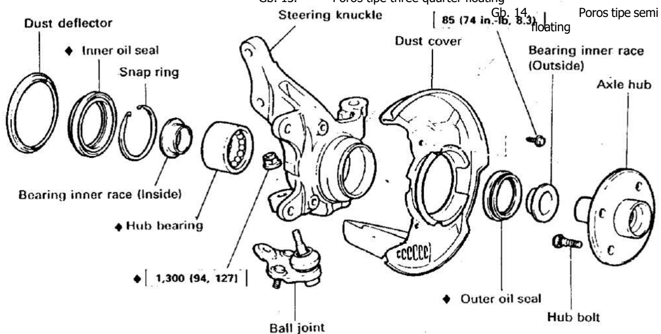
Gb. 13. Poros tipe three quarter floating
