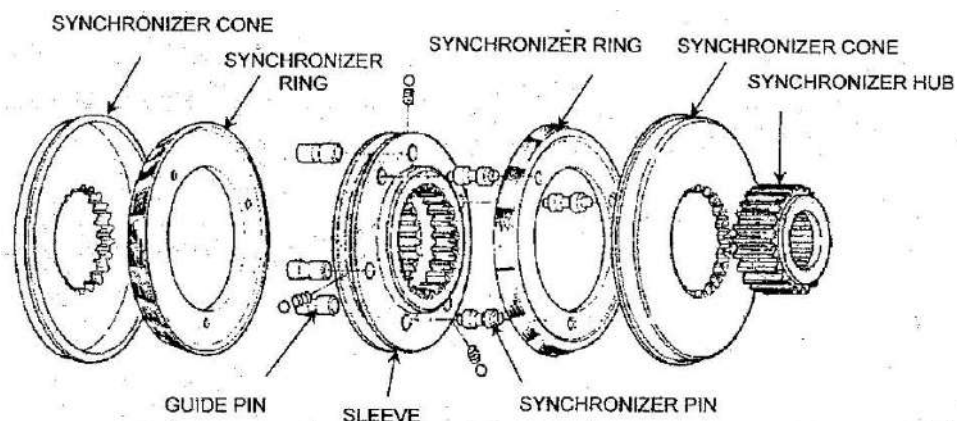
Gb. 1. Unit synchromesh model inertial lock pin
