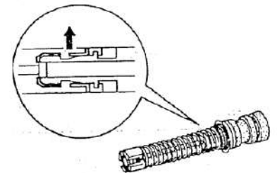
Gb. 10. Membongkar piston unit
