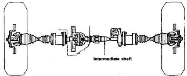
Gb. 2. Front axle (intermediate type)
