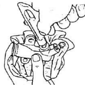
Gb. 17. Release silinder dan release fork
