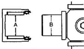
Gb. 27. Memeriksa diameter bantalan spider
