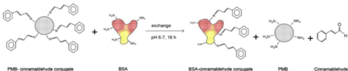
Fig. 5. Mechanism of exchange reaction between imine conjugates of PMB-cinnamaldehyde and amino groups of serum albumin.
