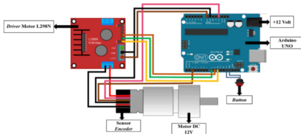
Gambar 3. Wiring hardware .
