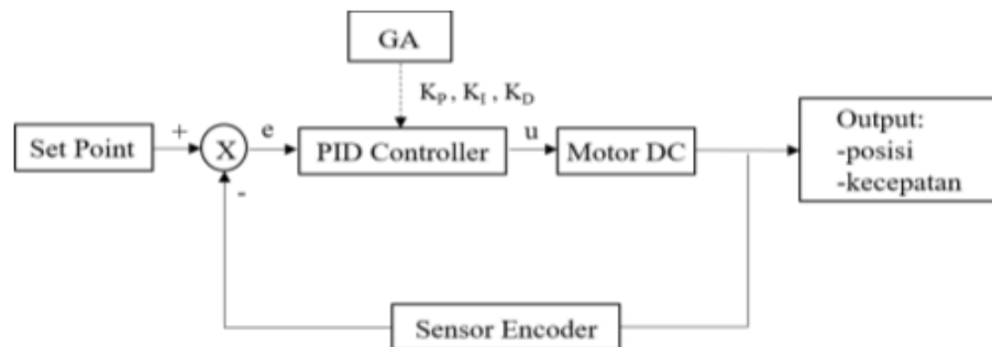
Gambar 1. Diagram blok tuning pengendali PID.
