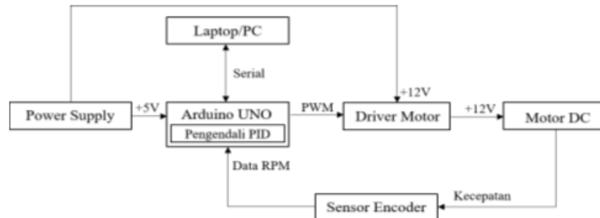
Gambar 2. Diagram blok hardware .
