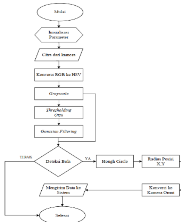
Gambar 2. Flowchart Sistem
