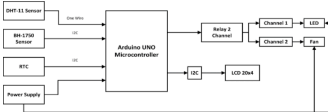
Figure 3. System block diagram
