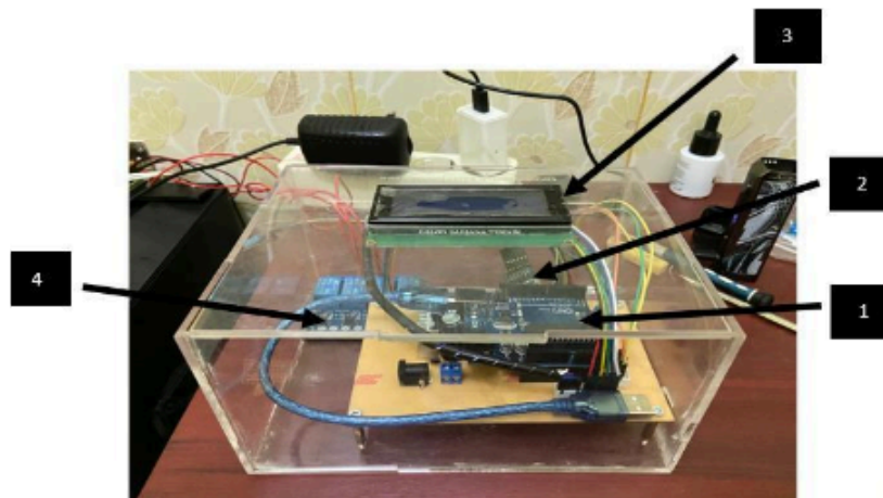
Figure 4. Controller box
