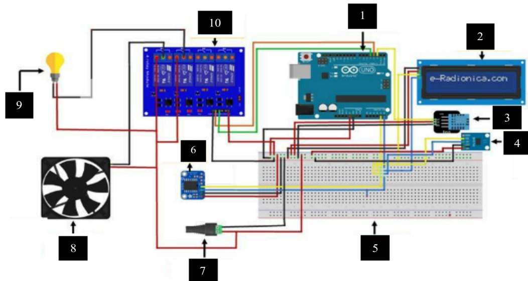
Figure 1. Schematic design of the system circuit
