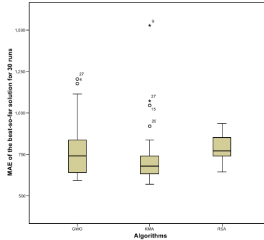
Fig. 2. Best solution diversity analysis for DS5
