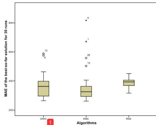
Fig. 1. Best solution diversity analysis for DS4
