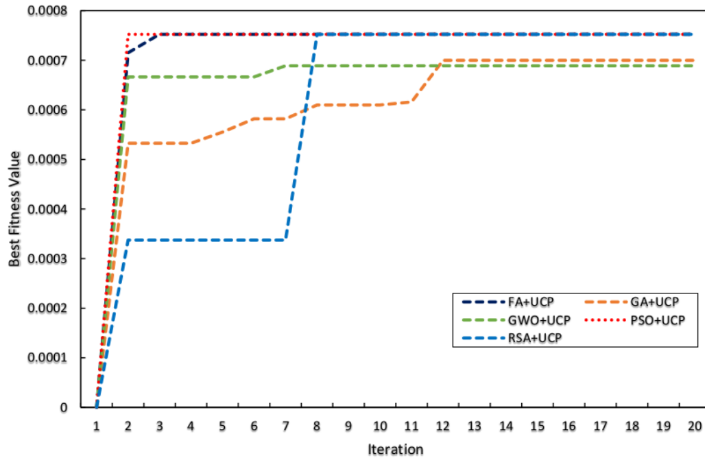
Figure 5. Convergence behavior comparison of all optimization methods
