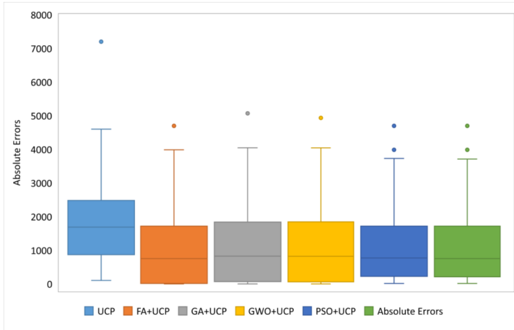
Figure 6. Best solution diversity analysis of all models
