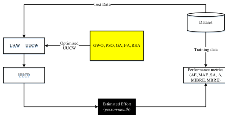
Figure 2 Experimental design flow
