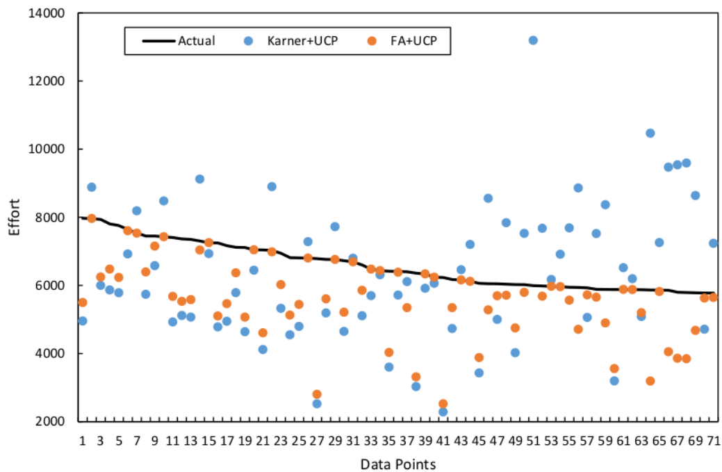
Figure 4. The plot showing both the actual and estimated effort values between FA+UCP and Karner+UCP models
