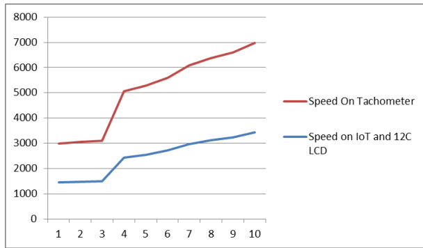
Fig. 7. Data test graph in High speed conditions
