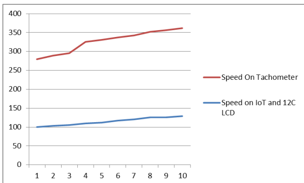
Fig. 7. Graph of test data in low speed conditions
