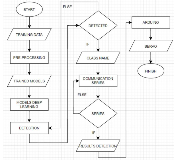
Figure 3. Flowchart
