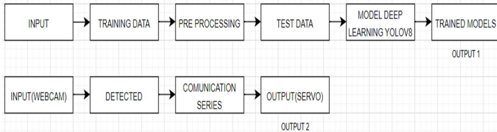
Figure 2. block diagrams
