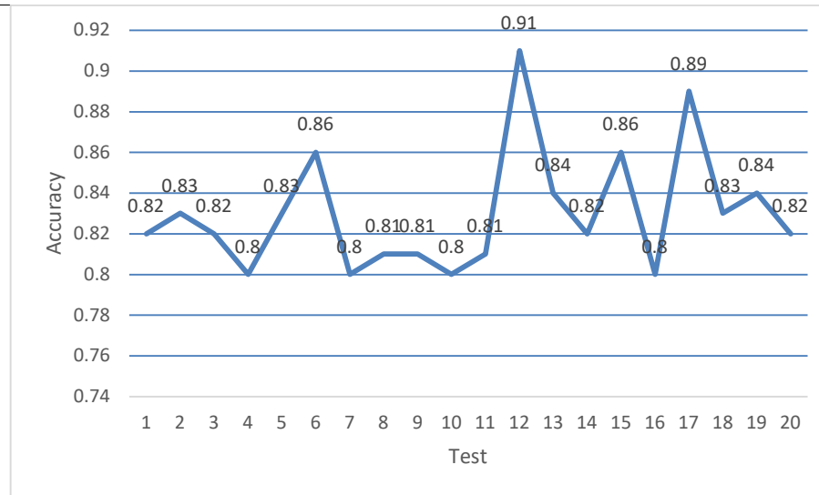
Figure 10. Grafic accuracy
