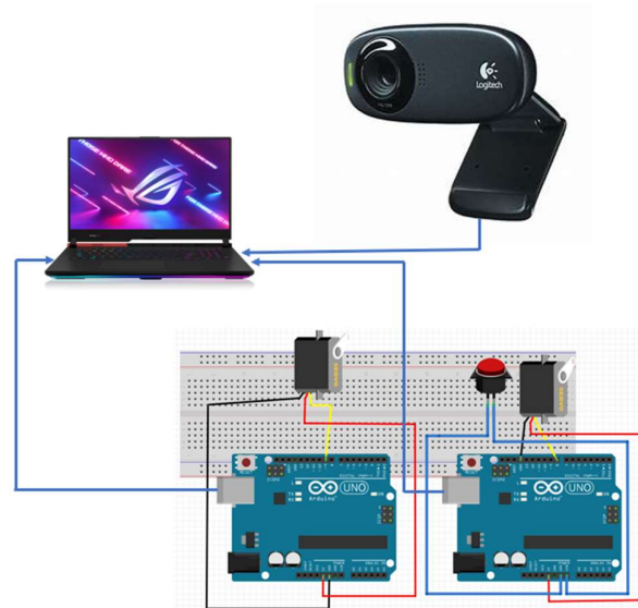
Figure 3. wiring detection and move servo
