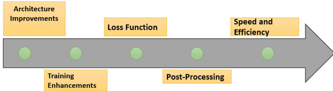
Figure 1.method yolov8 detection
