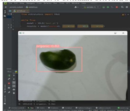
Figure 6. implementation
