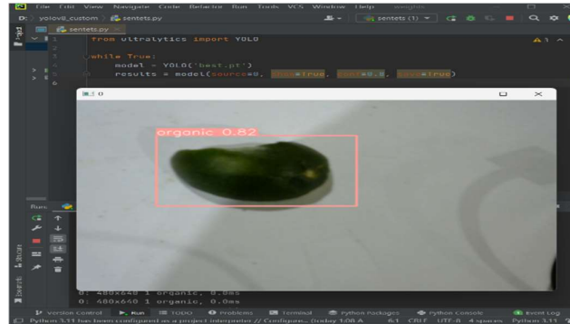
Figure 9. object detection
