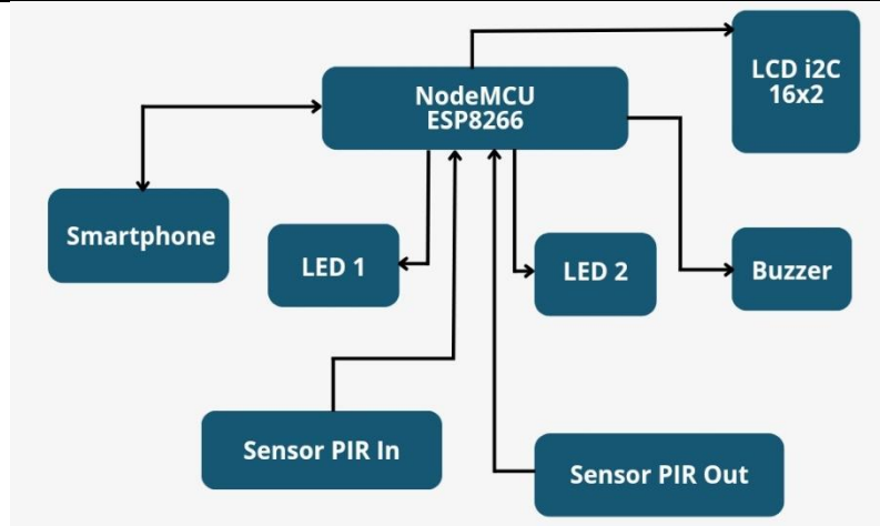
Figure 4. Block diagram
