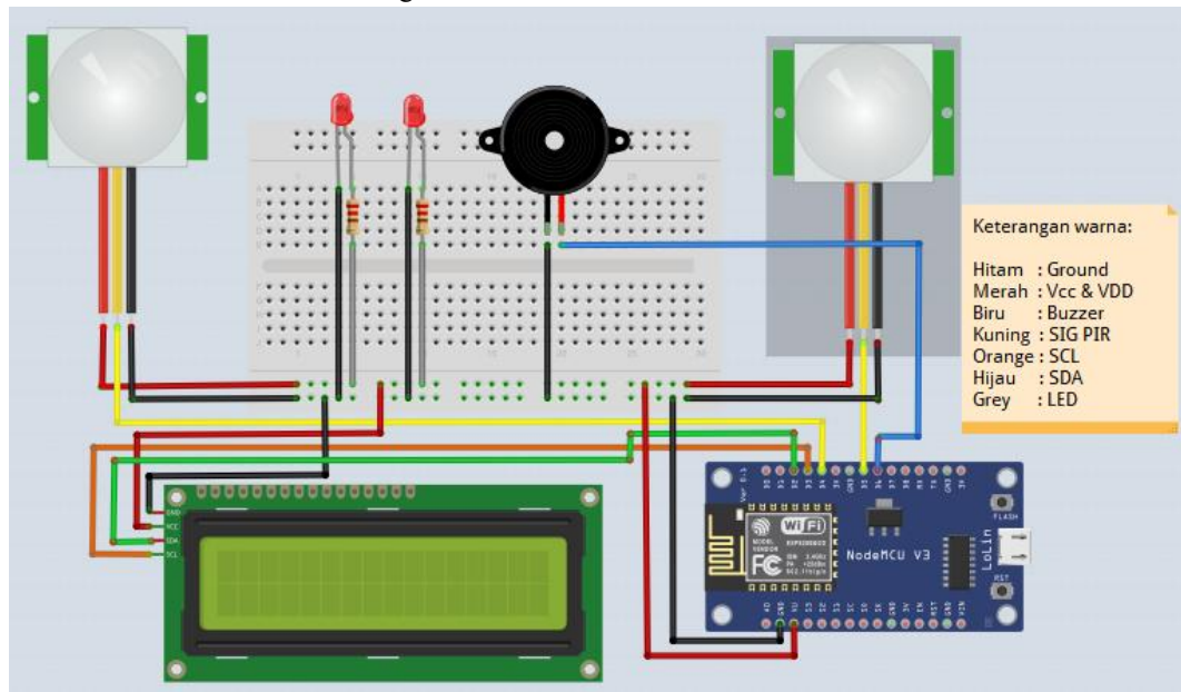
Figure 3. Wiring diagram
