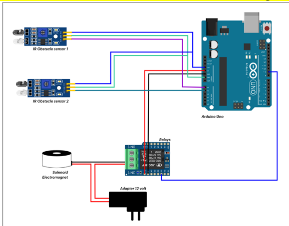
Figure 3. Scheme of automation device
