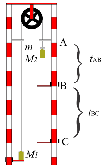
Figure 2. Working principle of Atwood Machine
