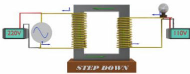
TRANSFORMATOR
