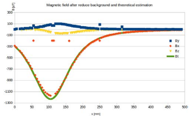
Fig. 8. The current-carrying magnetic field is reduced by the background magnetic field, compared with the theoretical obtained magnetic field based on equation 3.
