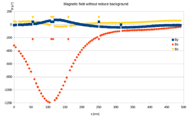
Fig. 7. The magnetic field when reverse current flows in the coil
