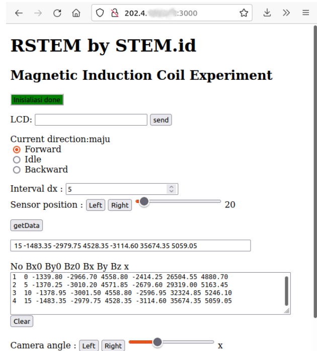
Fig. 4. GUI display running on the Firefox web-browser
