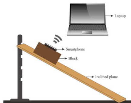
Figure 1. The Design of the Experiment
