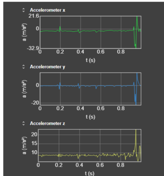
Figure 3. The Graph of Acceleration Towards Time Obtained from Phypox Application
