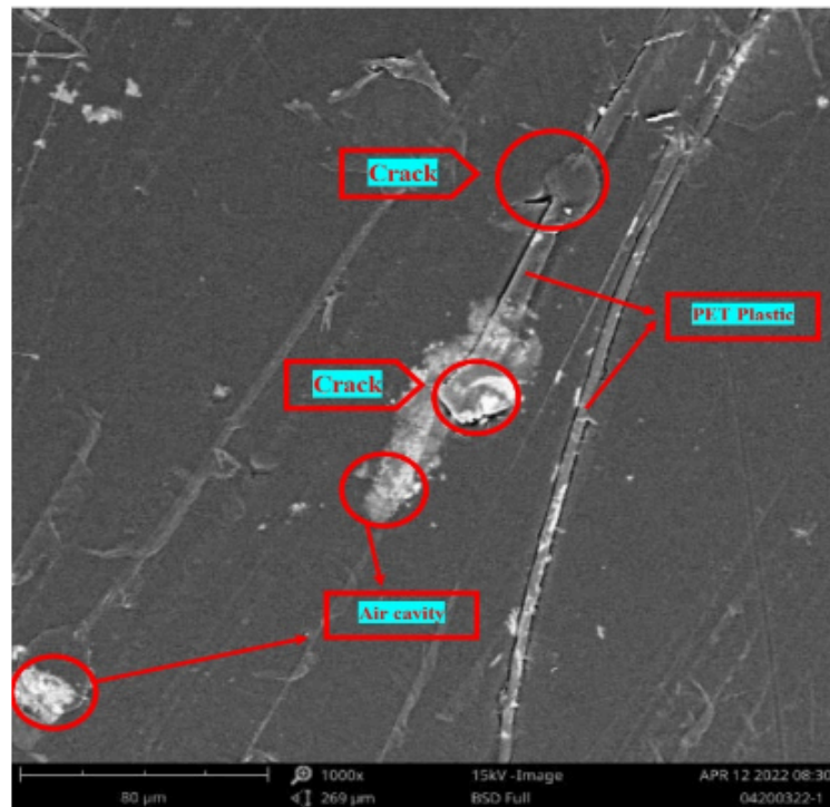
Figure 12. SEM image of eco-brick material.
