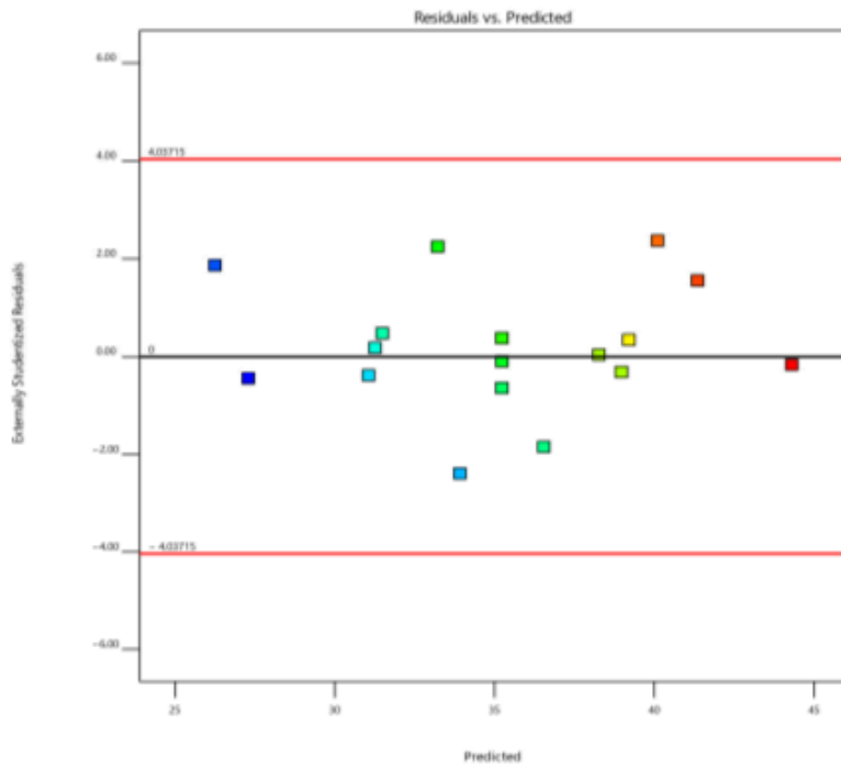
Figure 6. Residual vs. predicted values.
