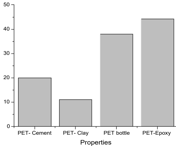
Figure 13. Compressive strength comparison of eco-bricks.
