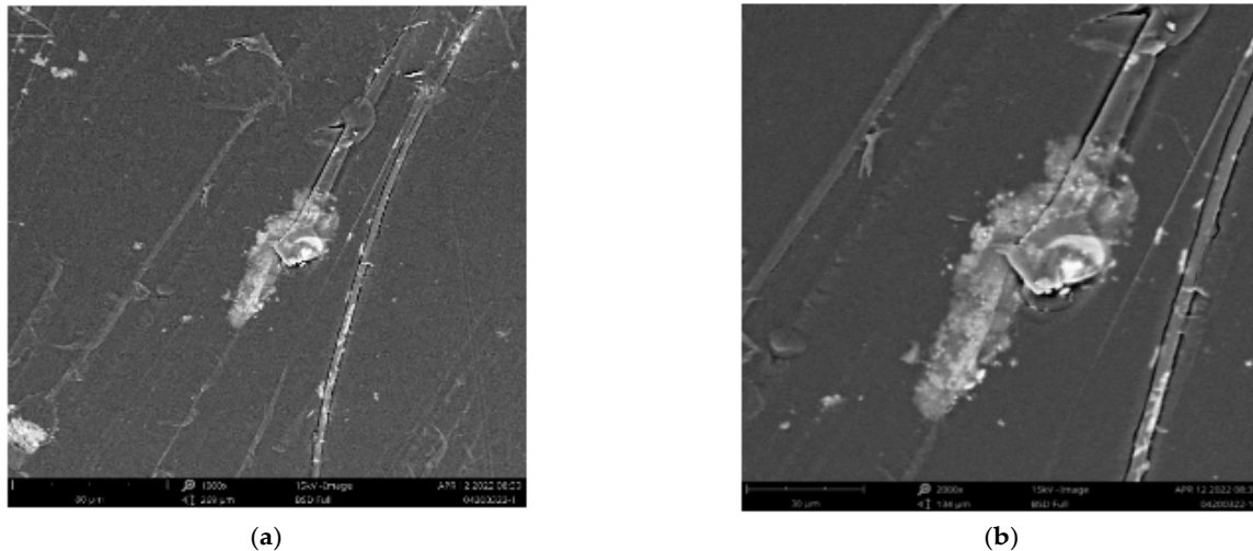
Figure 11. SEM images—1000 \times magnification and 2000 \times magnification. (a) SEM analysis of an eco-brick; magnification 1000 \times . (b) SEM analysis of an eco-brick; magnification 2000 \times .
