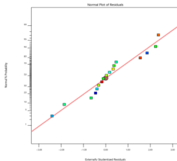
Figure 4. Normal probability vs. external residual plot.
