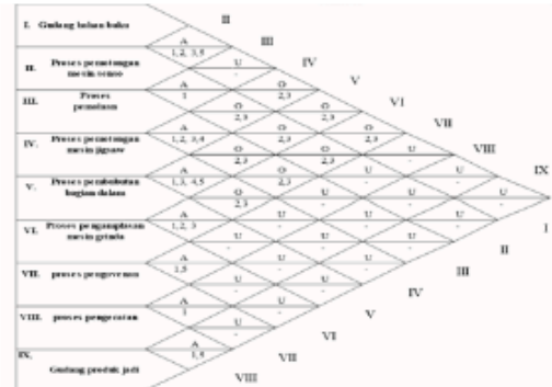
Gambar 2 Activity Relationship Chart Produk Sendok Kayu
