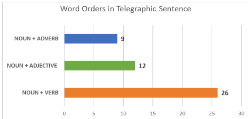
Figure 2. Word Orders in Telegraphic Sentence
