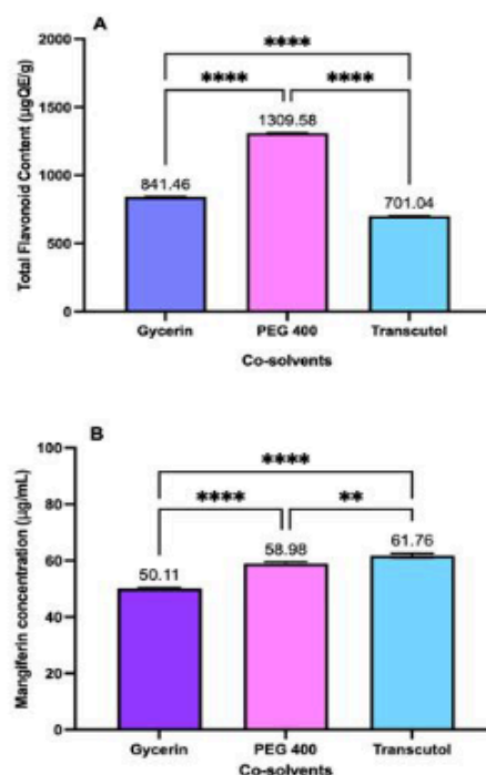
Figure 5. Quantitative analysis of (A) Total Flavonoid Content and (B) Mangiferin Concentration in different co-solvent solutions
