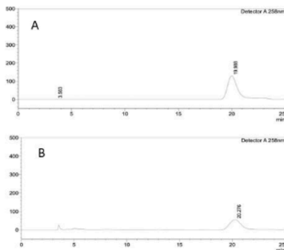
Figure 4. The chromatographic profile of the standard mangiferin (A) and sample (B) exhibits the retention time of mangiferin
