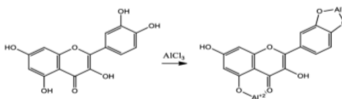
Figure 1. Formation of complexes through a reaction between hydroxyl groups present in flavonoids and aluminum chloride ( \text{AlCl}_3 )
