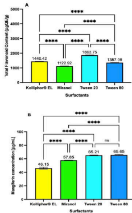
Figure 3. Quantitative analysis of Total Flavonoid Content (A) and Mangiferin Concentration (B) in different surfactant solutions
