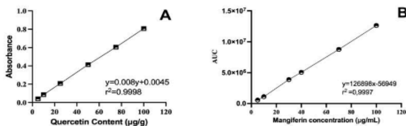
Figure 2. The standard curve for quercetin (A) and mangiferin (B)
