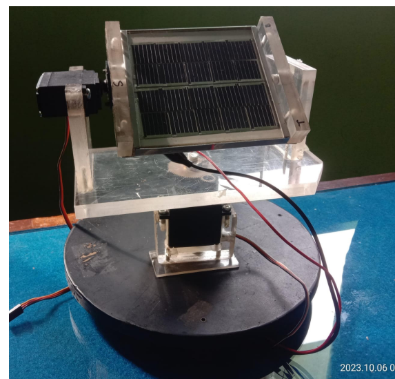
Figure 3. Apparatus for experiments on light energy with two axis solar tracker
