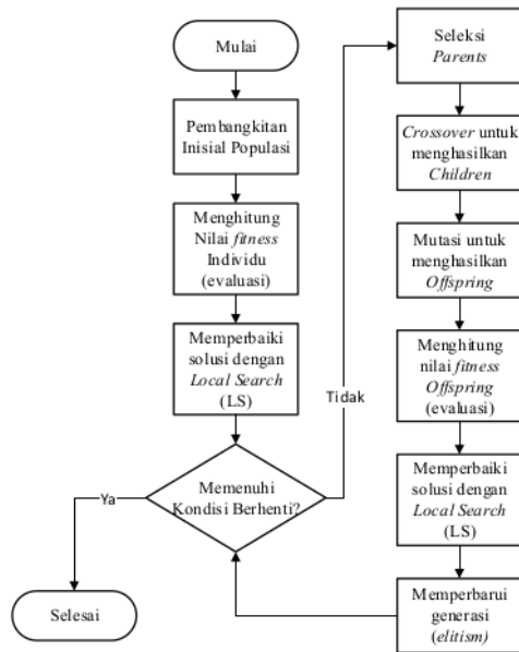
Gambar 1. Diagram Alir Tahapan Hybrid GA
